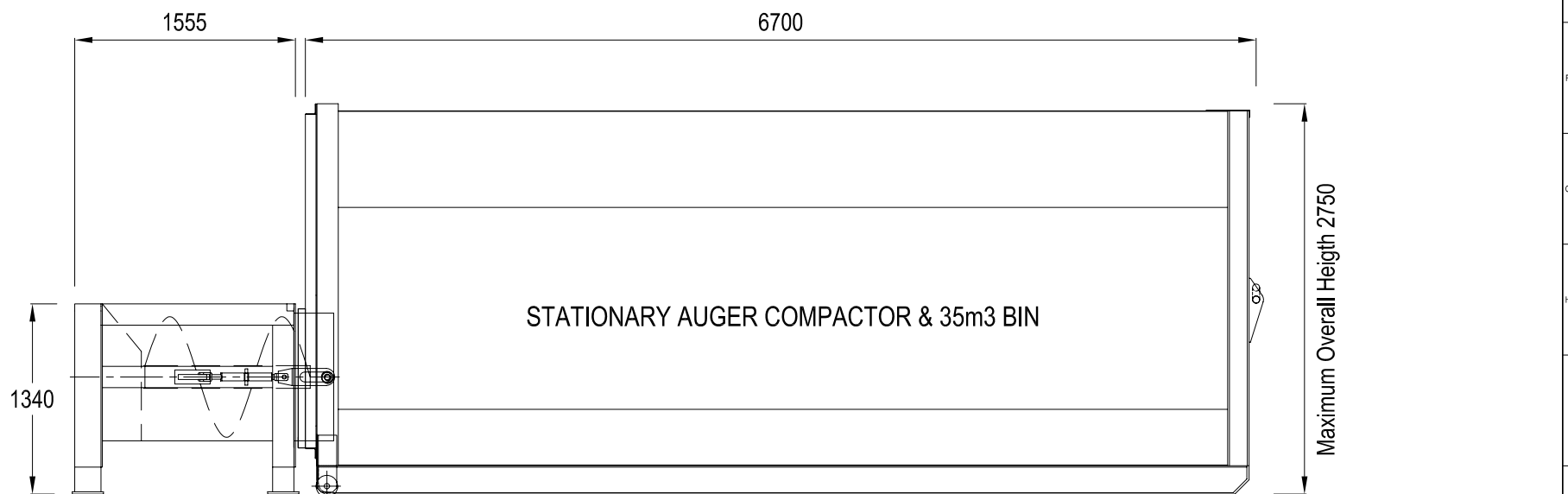
SIDE VIEW
