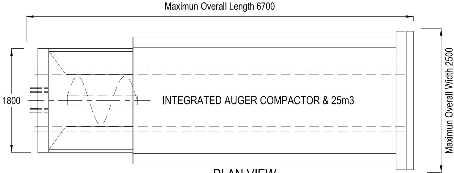
PLAN VIEW
