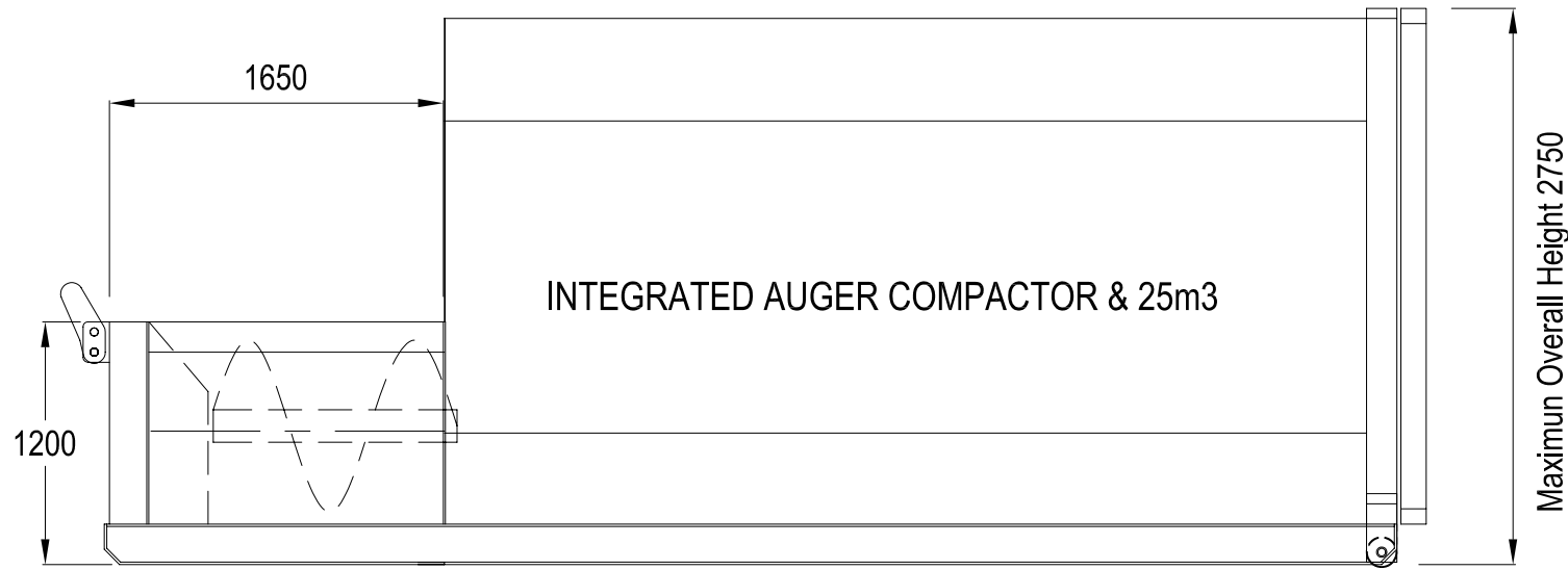
SIDE VIEW
